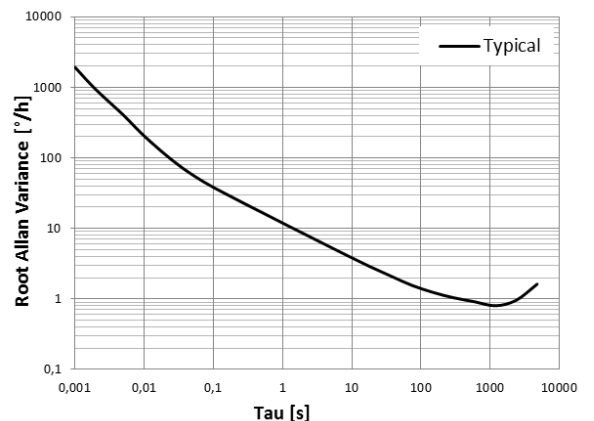
Figure 12 Allan variance
