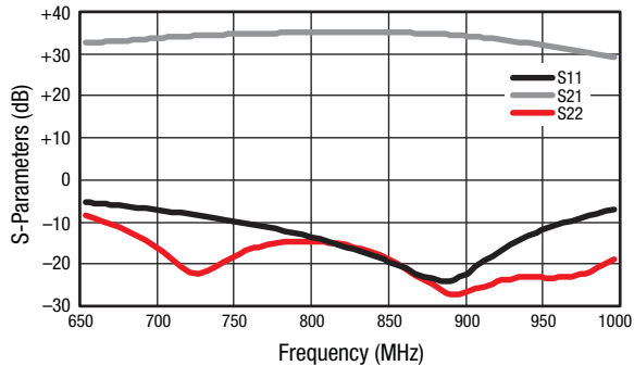
Figure 3. Small Signal Parameters vs Frequency
