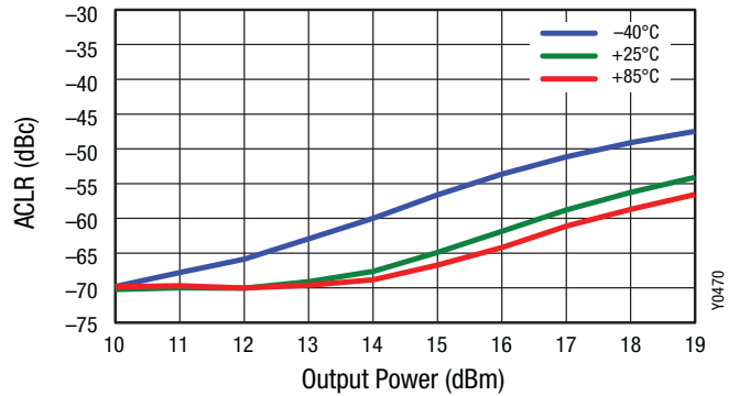
Figure 10. ACLR vs Output Power (WCDMA, TM1)
