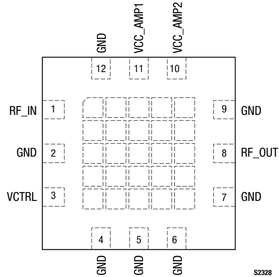
Figure 2. SKY65385-11 Pinout – 12-Pin MCM (Top View)
