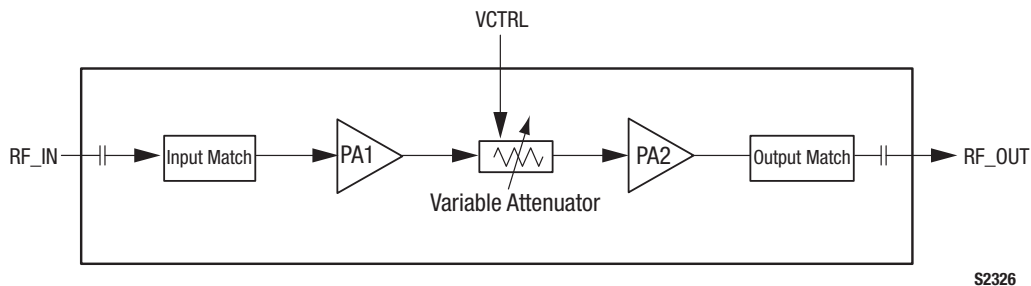
Figure 1. SKY65385-11 Block Diagram
