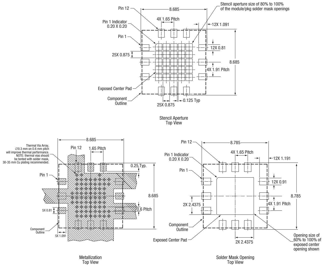
Figure 17. SKY65385-11 PCB Layout Footprint
