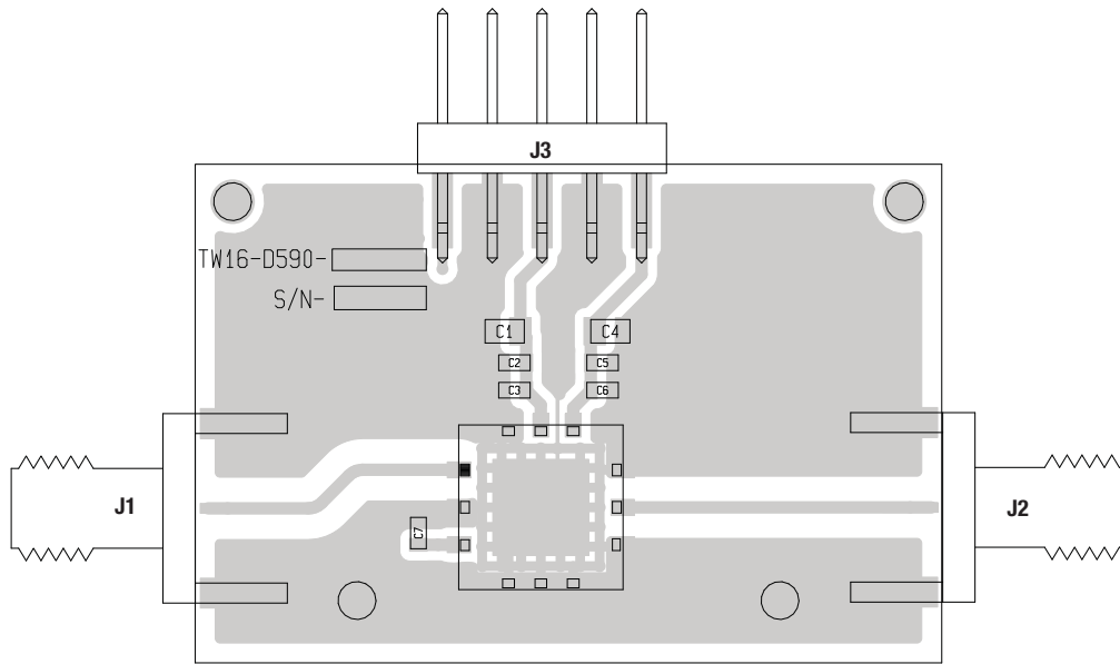
Figure 14. SKY65385-11 Evaluation Board Assembly Drawing
